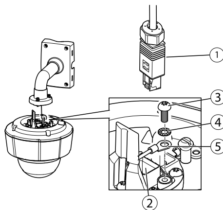
1. Network connector – RJ45 Push-pull Connector (IP66)
