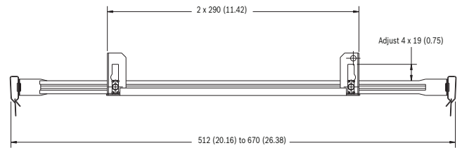
VGA-IC-SP dimensions
