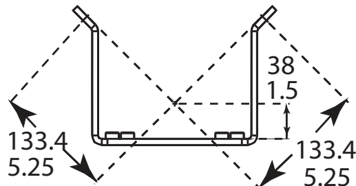
VG4-A-9541_Pole-Mount-Adapter_dimensions
