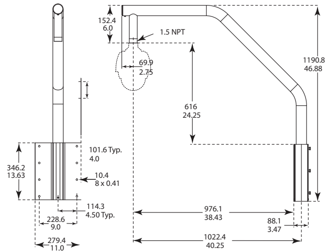
VGA-ROOF-MOUNT dimensions
