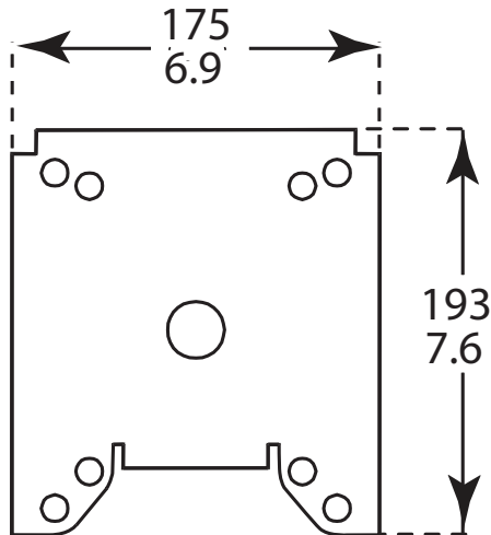
VG4-A-9541_Pole-Mount-Adapter_dimensions
