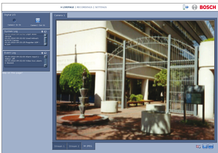
Figure 3.1: Live page
