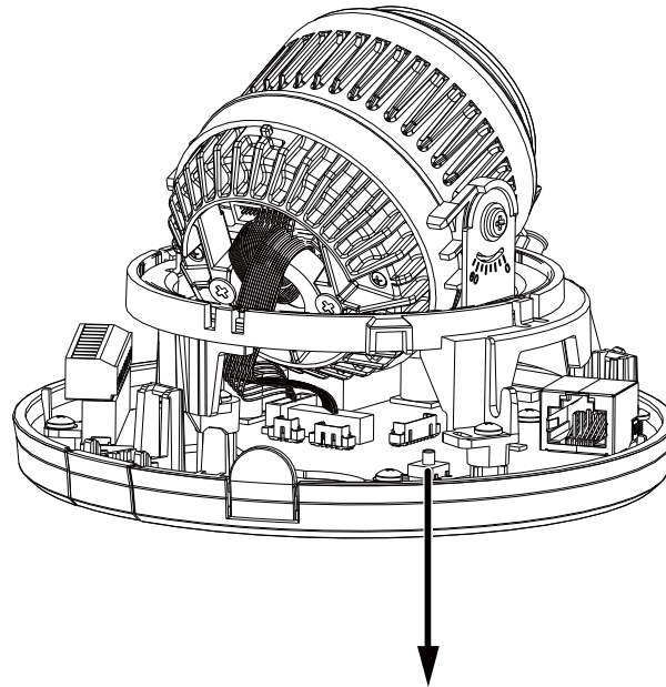
Reset Button
