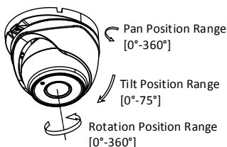
Figure 2-10 3-axis Adjustment
