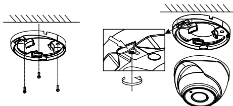
Figure 2-9 Install the Turret Camera
