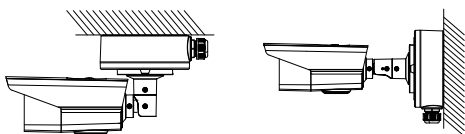
Figure 2-6 Fix the Camera to the Ceiling/Wall
