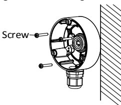
Figure 2-5 Fix the Camera to the Ceiling
