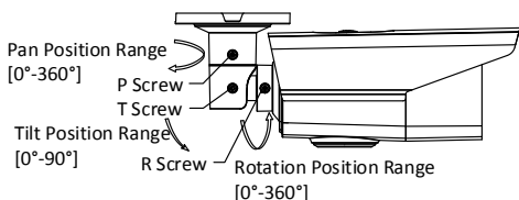
Figure 2-3 3-axis Adjustment
