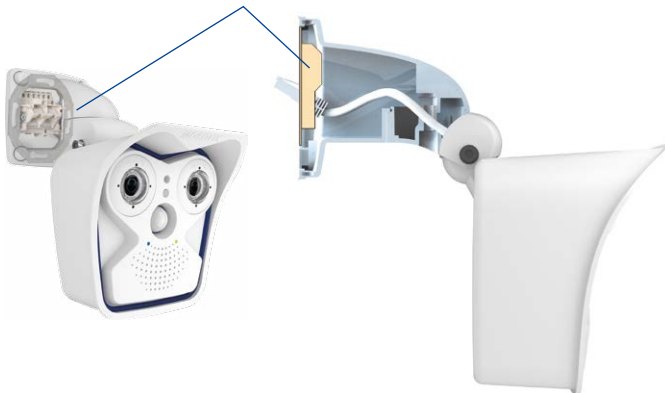
Space for RJ45 in-wall socket/concealed cabling
