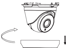
Figure 2-2 Remove the trim ring
