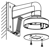
Figure 2-14 Install the Adapter to the Pendant Cap
