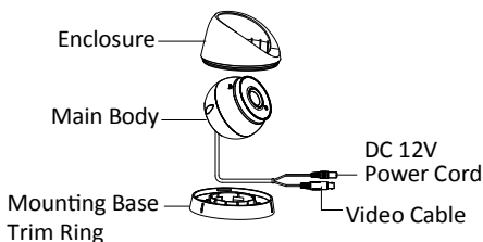
Figure 1-1 Overview of Type I Camera
