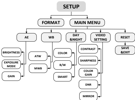
Figure 3-1 Main Menu Overview
