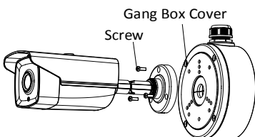
Figure 2-9 Fix the Camera with the Gang Box
