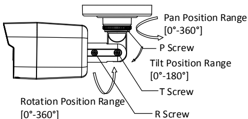
Figure 2-2 3-axis Adjustment
