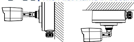
Figure 2-5 Fix the Camera to the Ceiling/Wall
