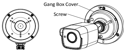
Figure 2-3 Fix the Camera with the Gang Box
