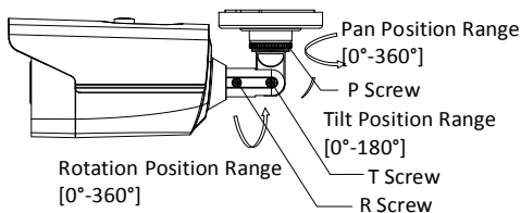
Figure 2-7 3-axis Adjustment
