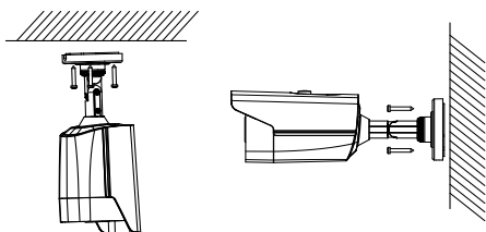
Figure 2-6 Fix the Camera to the Ceiling/Wall
