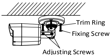
Figure 2-1 Fix the Camera to the Ceiling
