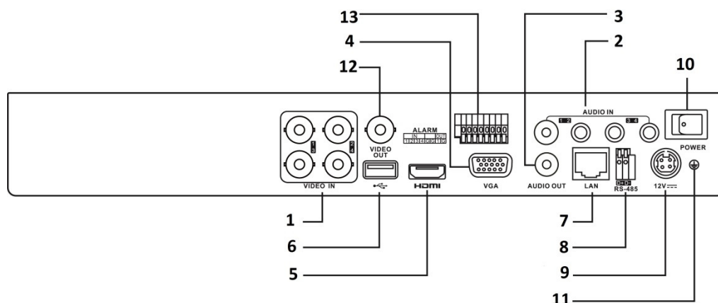
Figure 1, DS-7204HUHI-F1/N - (DS-7208HUHI-F2/N and DS-7216HUHI-F2/N provide 8 and 16 video input interfaces respectively) -
