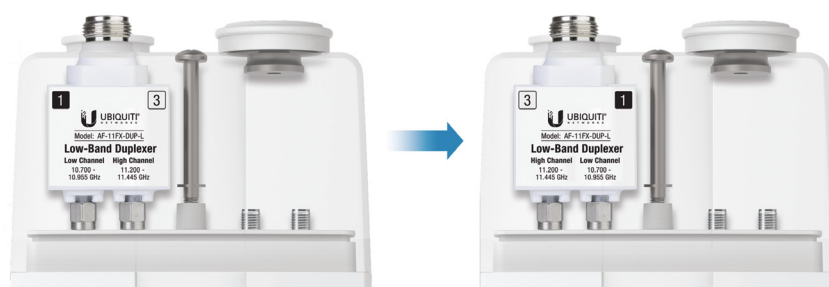
Reversible Duplexers For Easy Channel Configuration
