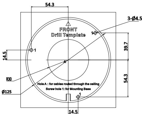
Figure 2-25 Drill Template
