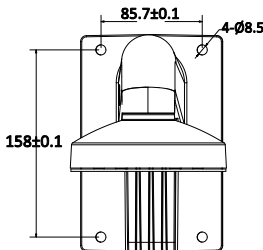
Figure 2-30 Dimension of Demonstrated Wall Mounting Bracket
