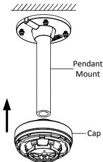
Figure 2-35 Install the Cap
