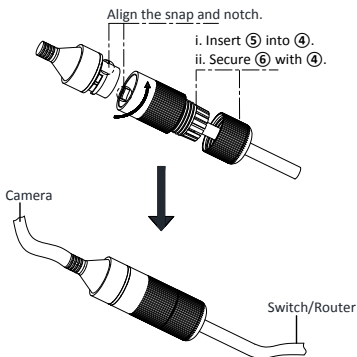
Figure 2-38 Water-proof Accessory Installation
