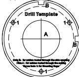
Figure 2-15 Drill Template of the Junction Box
