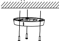
Figure 2-3 Attach the Mounting Base to the Ceiling
