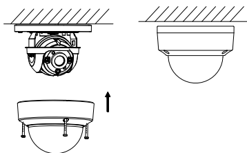
Figure 2-23 Bubble Reinstallation
