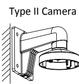
Figure 2-17 Install the Bracket
