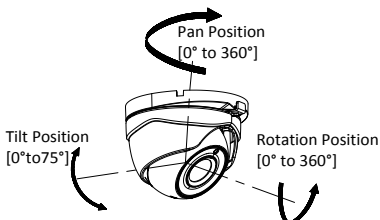
Figure 2-14 3-axis Adjustment
