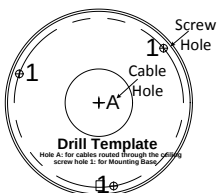
Figure 2-19 Drill Template
