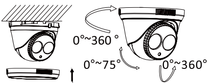
Figure 2-6 3-axis Adjustment
