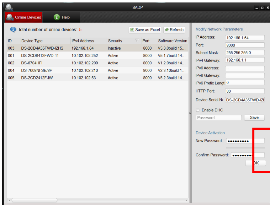
Figure 21 Password Field with "Risky" Unacceptable Password
