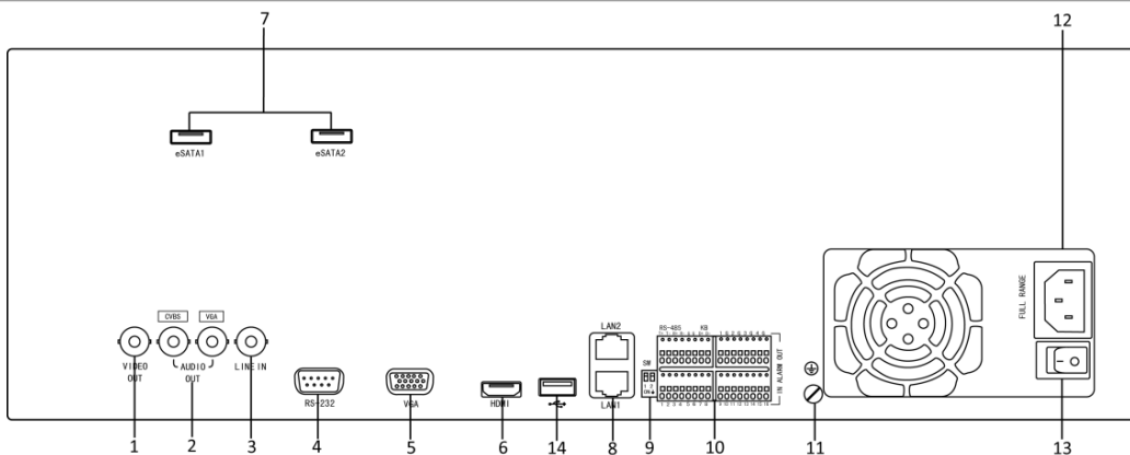
Figure 7 DS-9600NI-XT
