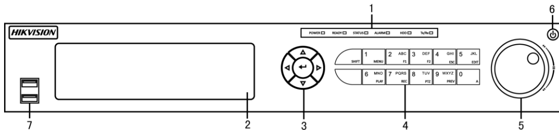
Figure 12 7700 NVR Front Panel Controls
