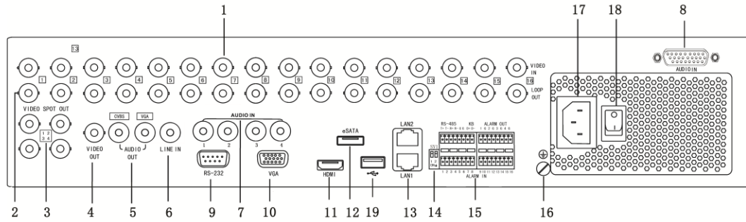
Figure 5 DS-9000HWI-ST & DS-9000HFI-RT
