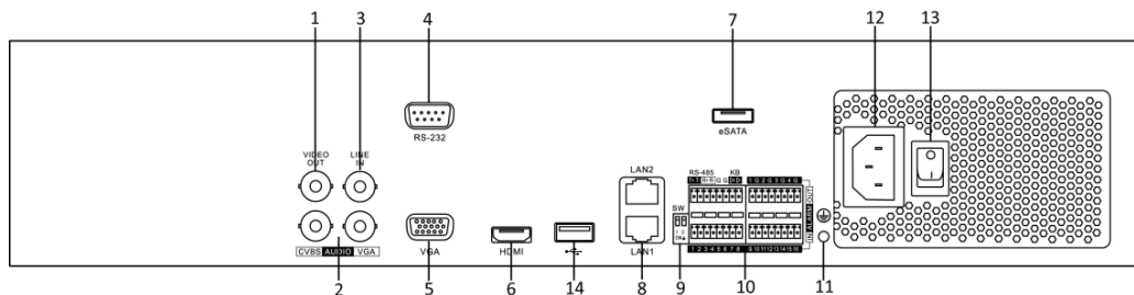
Figure 6 DS-9600NI-ST/RT
