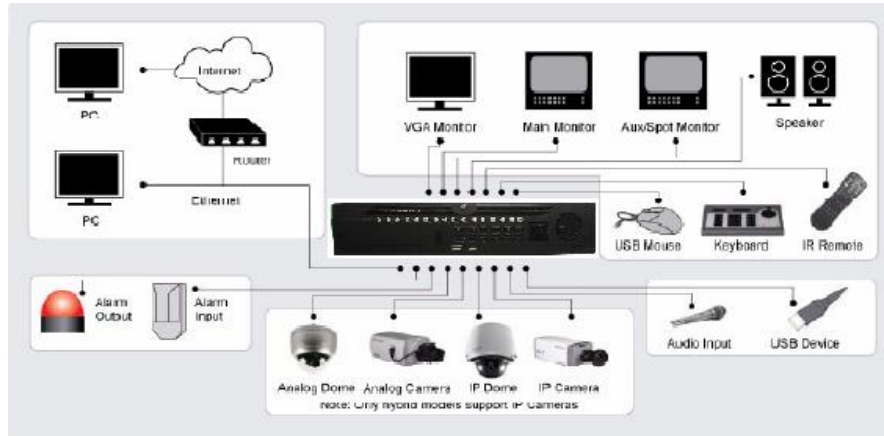
Figure 9 Product Application Diagram
