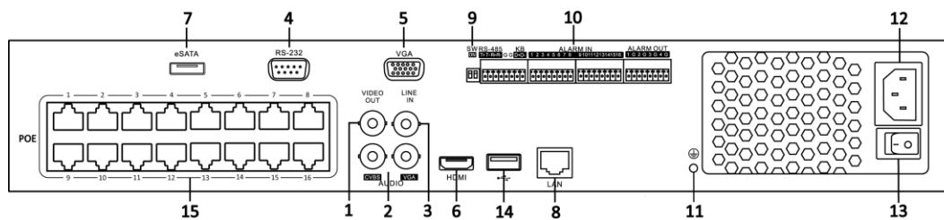
Figure 8 DS-7700NI-SP
