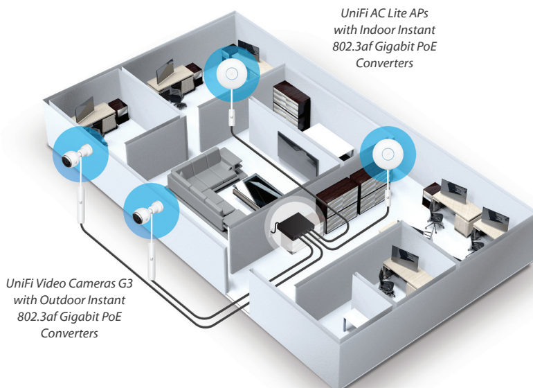
Indoor and Outdoor Products Powered by 802.3af Switch
