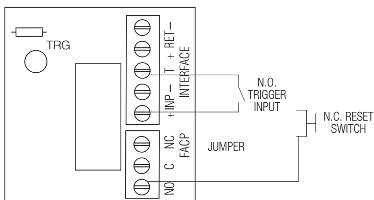
Fig. 13 Normally Open FACP Latching trigger input with reset: (This output has not been evaluated by UL)
