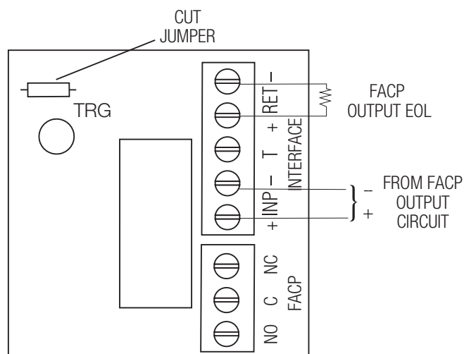
Fig. 13 Normally Open FACP Latching trigger input with reset: (This output has not been evaluated by UL)
