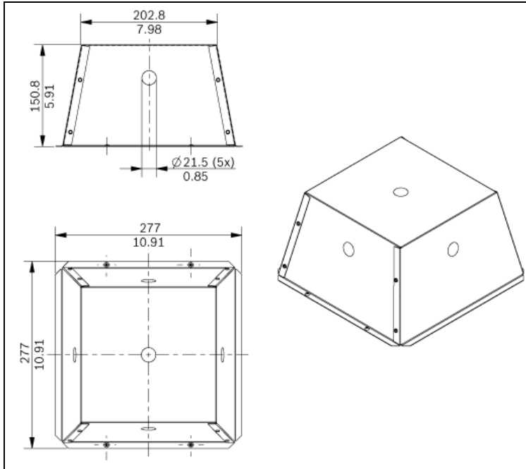
LM2-BB Back Box
