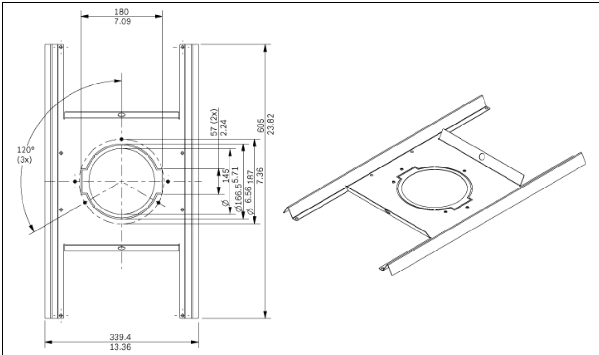
LM2-TB Tile Bridge
