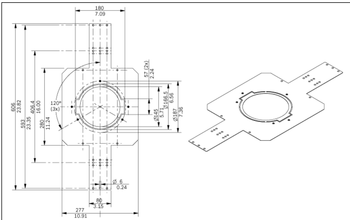
LM2-PMR Plaster Mounting Ring
