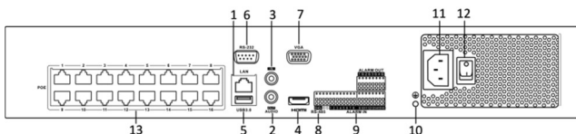
DS-7732NI-I4/16P
