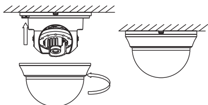
Figure 2-3 Complete the Installation
