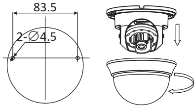
Figure 2-1 The Disassembling
