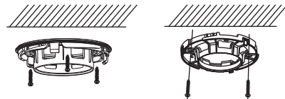
Figure 2-6 Secure the Mounting Base
