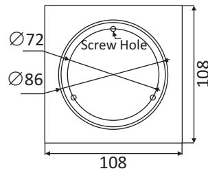
Figure 2-4 Drill Template of Type II Camera
