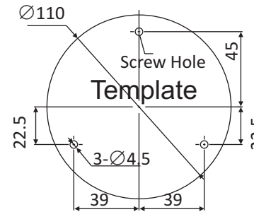
Figure 2-9 The Drill Template
