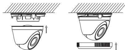
Figure 2-7 Secure the Components
