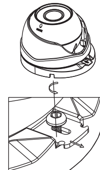
Figure 2-10 The Lock Screw
