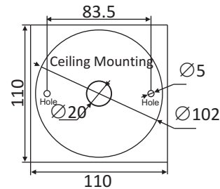
Figure 2-5 Drill Template of Type III Camera
