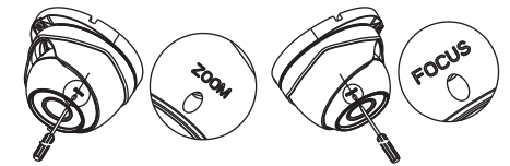
Figure 2-12 Zoom and Focus Adjustment
