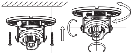
Figure 2-2 The Securing & 3-axis Adjustment
