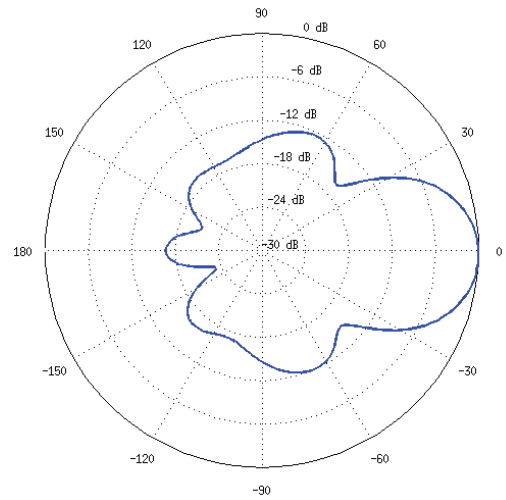
Horizontal Elevation
