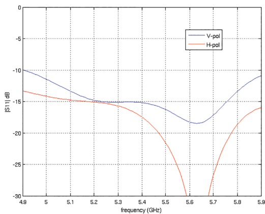
Return Loss
