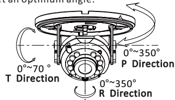
Figure 2-4 3-axis Adjustment
