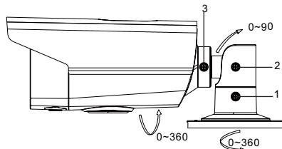
Figure 2-7 3-axis Adjustment
