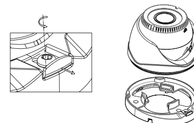
Figure 2-2 Remove the Clip Plate
