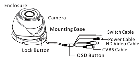
Figure 1-1 Overview of Type I Camera
