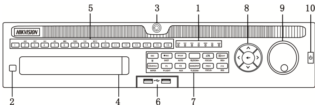
Figure 10 9000HQHI-SH Panel Controls
