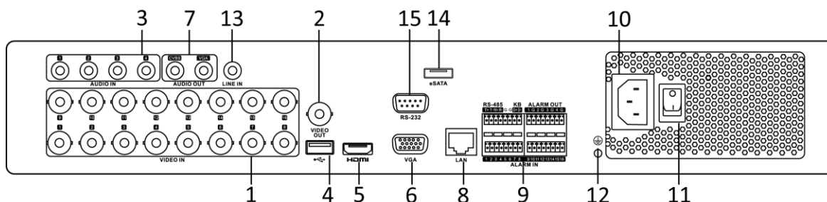
Figure 5 DS-7316HQHI-SH
