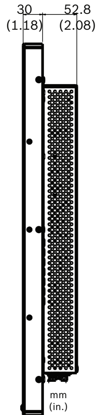
UML-423-90/UML-553-90: Side View
