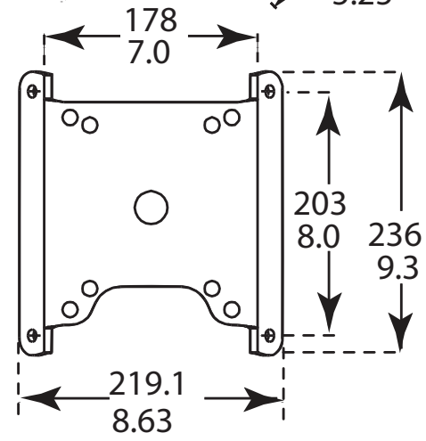
VG4-A-9542_Corner-Mount-Adapter_dimensions
