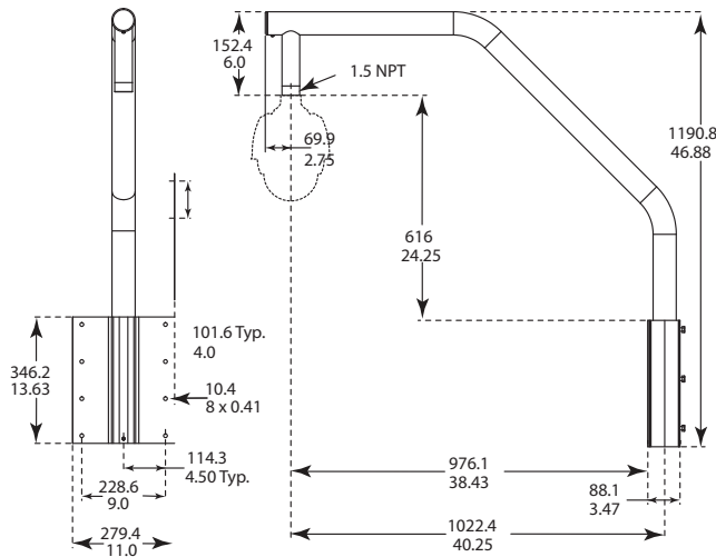
VGA-ROOF-MOUNT dimensions
