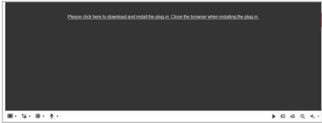
Figure 4-2 Download Plug-in
