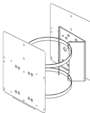
1x PBC-2 and x2 Adaptor Plates
