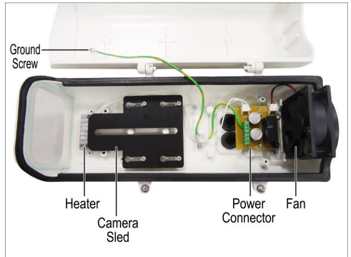
Housing with Heater and Fan
