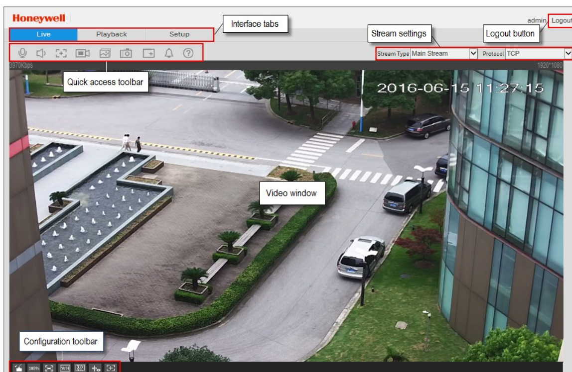
Figure 2-1 Live Interface
