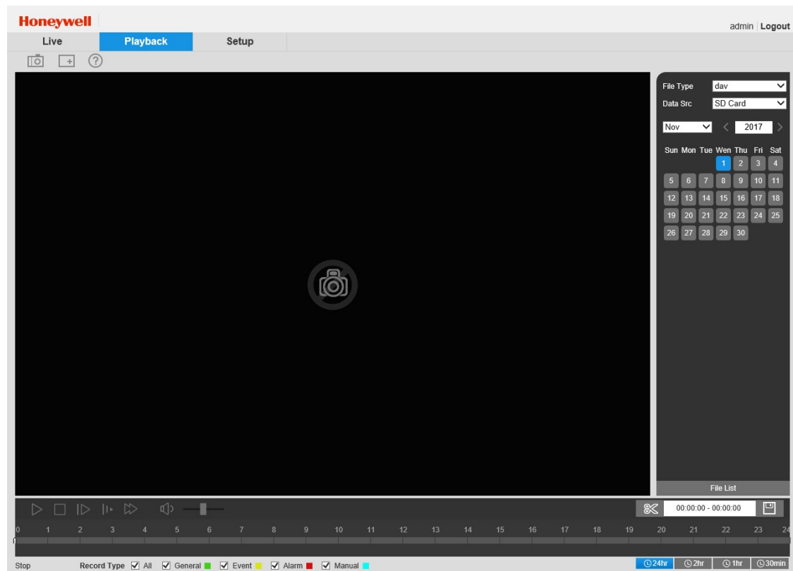
Figure 3-1 Playback Interface
