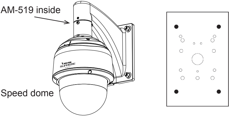
Use M8X25mm screws
