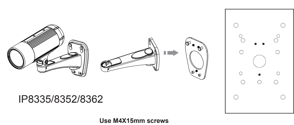
Use M4X15mm screws
