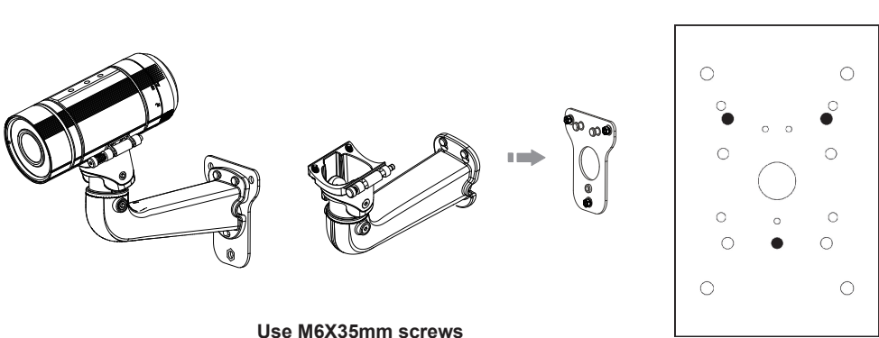
Use M6X35mm screws
