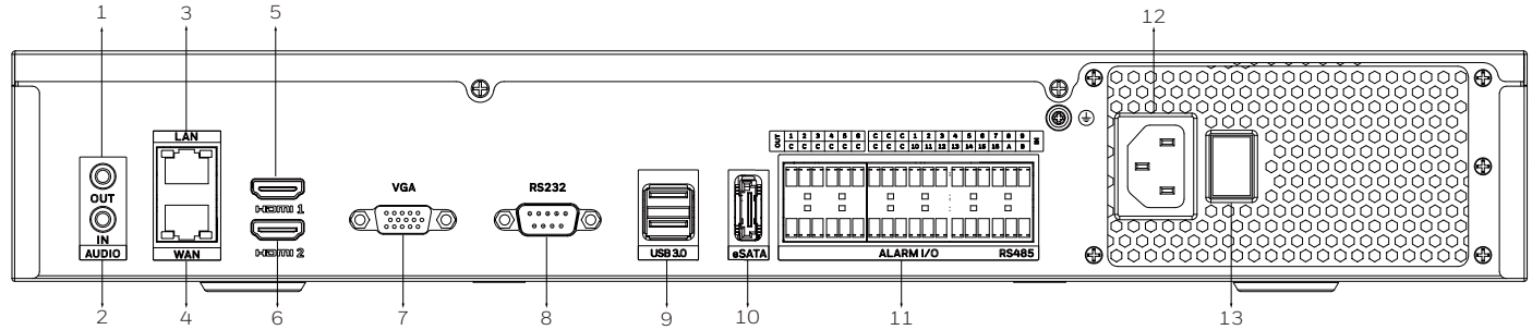
HN356404xxNR
