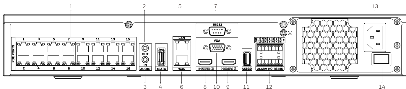
HN351604XXR
