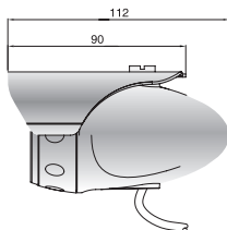
Figure 5.3 Side view
