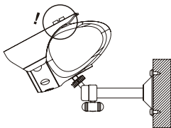
Figure 3.2 Camera mounted from bottom
