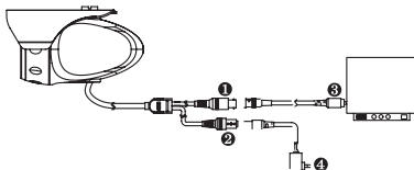
Figure 3.1 DIY cable connection
