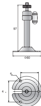
Figure 5.4 Mounting bracket
