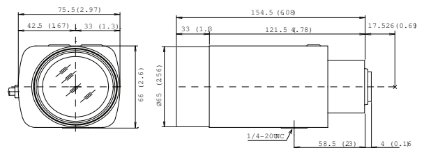
Dimensions LTC 3793/51
