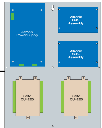
TSA1 - with one (1) Altronix Power Supply, two (2) Altronix Sub-Assemblies and two (2) Salto CU42E0
