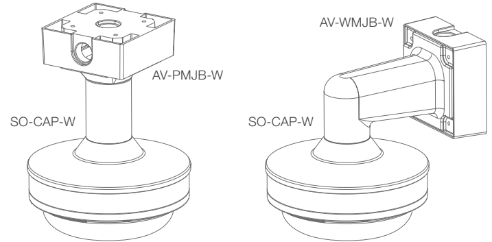
Ceiling Mount Configuration
